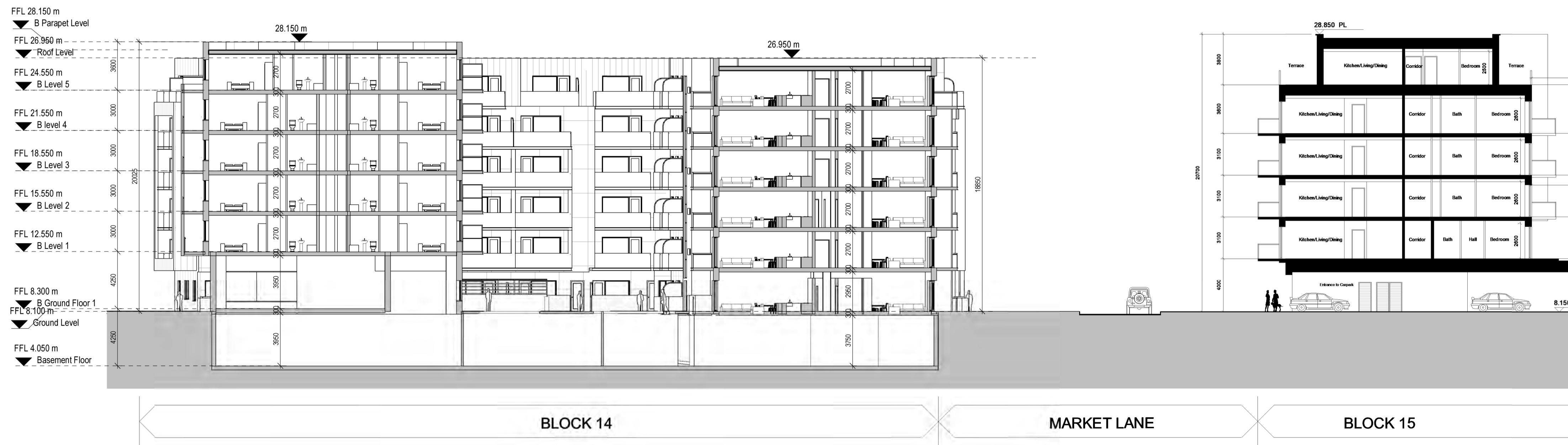
BLOCK 14 SECTION F-F Scale 1 : 200
